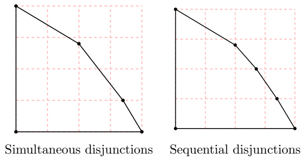
FIGURE 3. Difference between the simultaneous and sequential application of disjunctions (x_1 \leq 2) \vee (x_1 \geq 3) and (x_2 \leq 1) \vee (x_2 \geq 2) on P .
