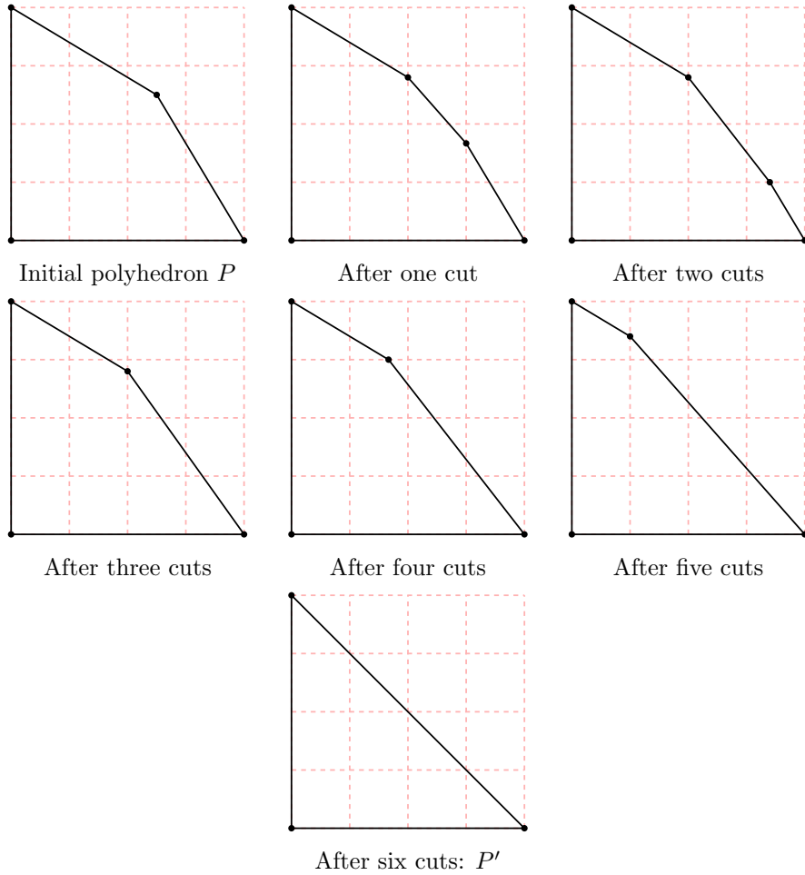
FIGURE 2. All stages of the application of the method on the example from [OM02]
