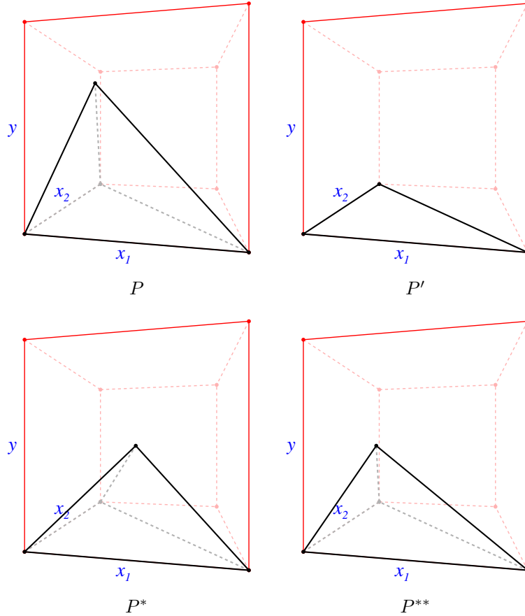
FIGURE 1. Polyhedra P , P' , P^* and P^{**} , in cubes 2 units wide
